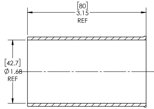
SECTION B-B EXPANDED SCALE 1:1
