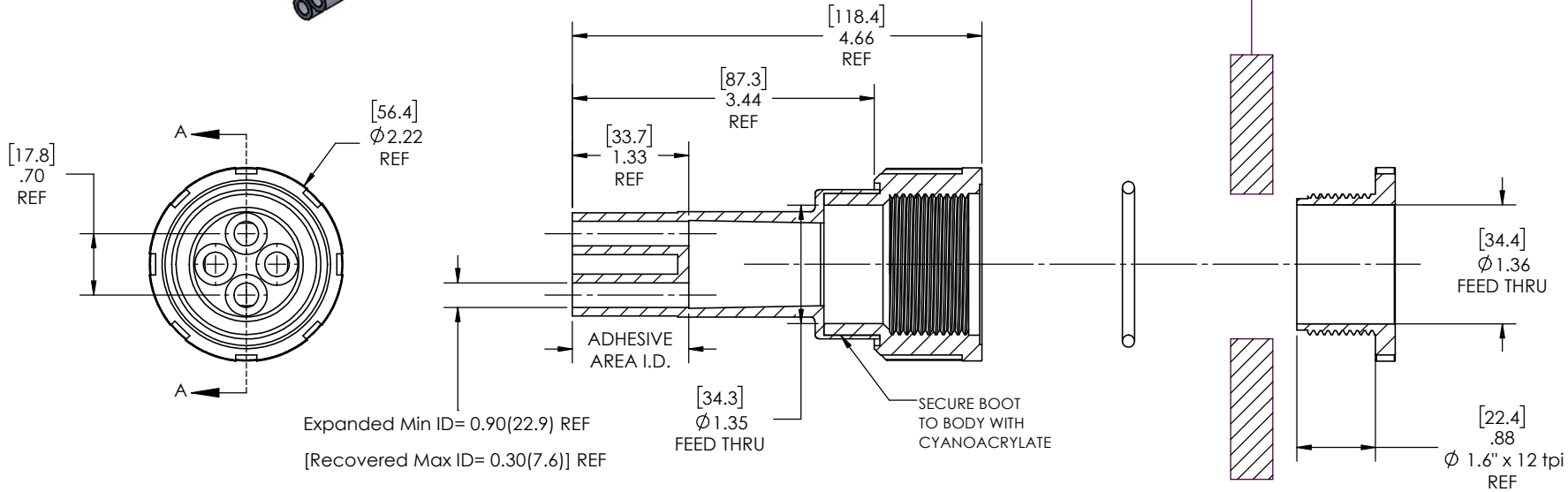
SECTION A-A RECOVERED SCALE 1 : 1.25
